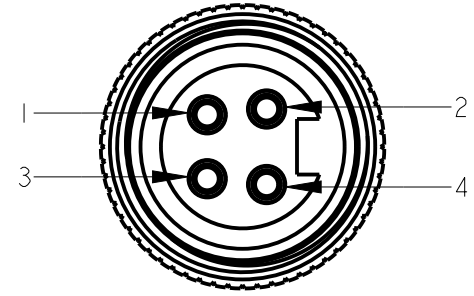
PINOUT
