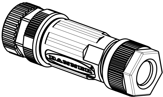
ISOMETRIC VIEW SCALE 3:2
