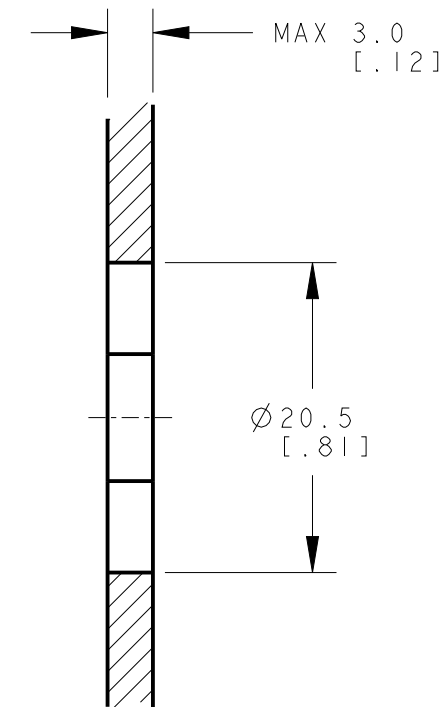
RECOMMENDED PANEL CUT-OUT
