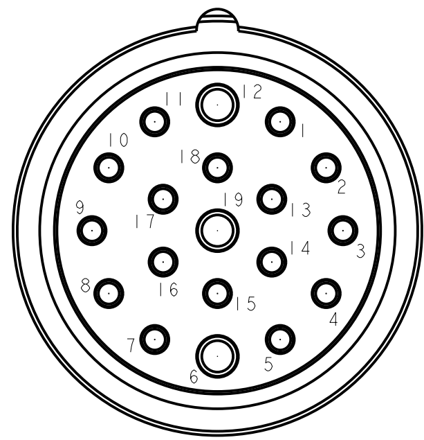
VIEW FROM FRONT (MALE) SCALE 4:1
