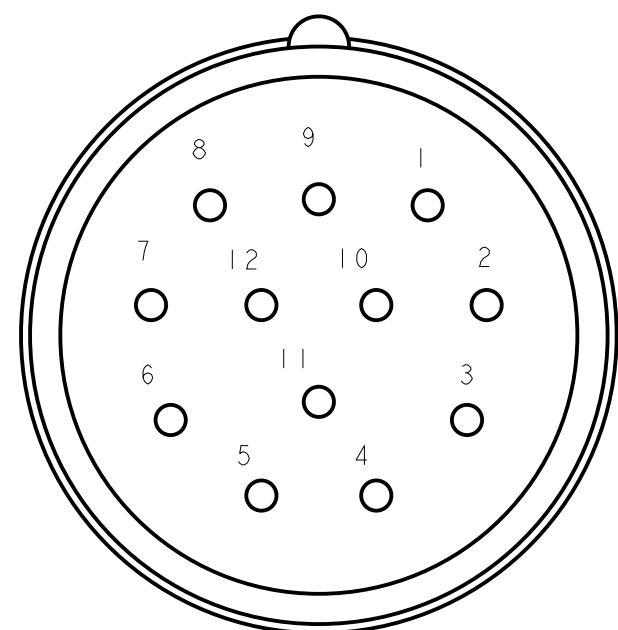
FRONT VIEW (MALE) SCALE 4:1
