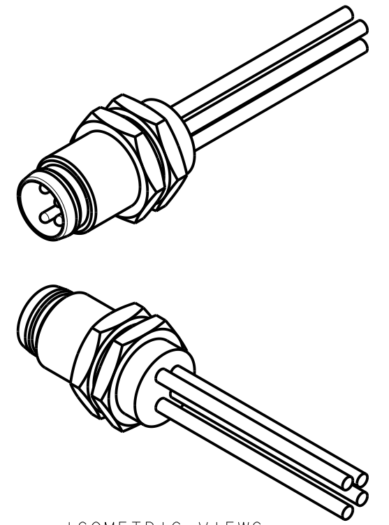
ISOMETRIC VIEWS
