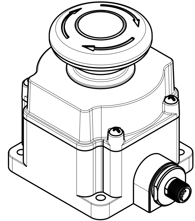
ISOMETRIC VIEW SCALE 3:4
