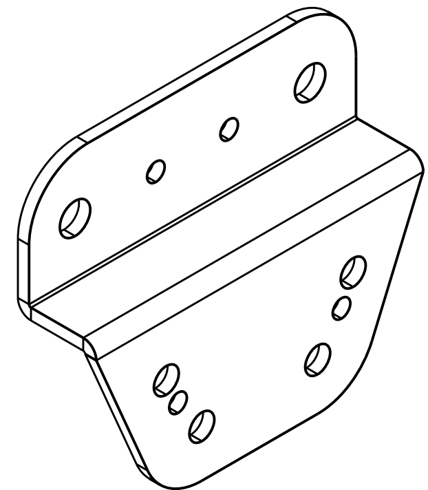
ISOMETRIC VIEW SCALE 1:1
