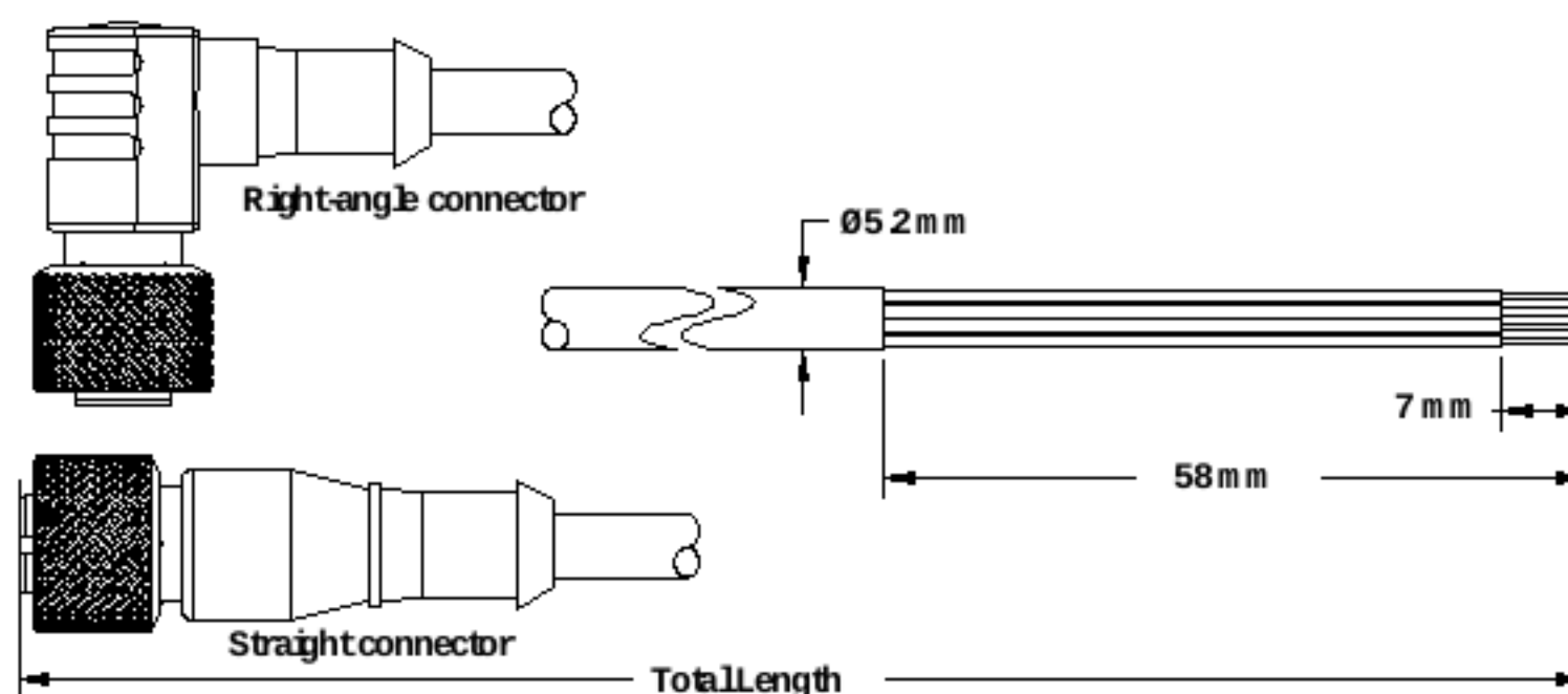
Figure 1. Wire dimensions
