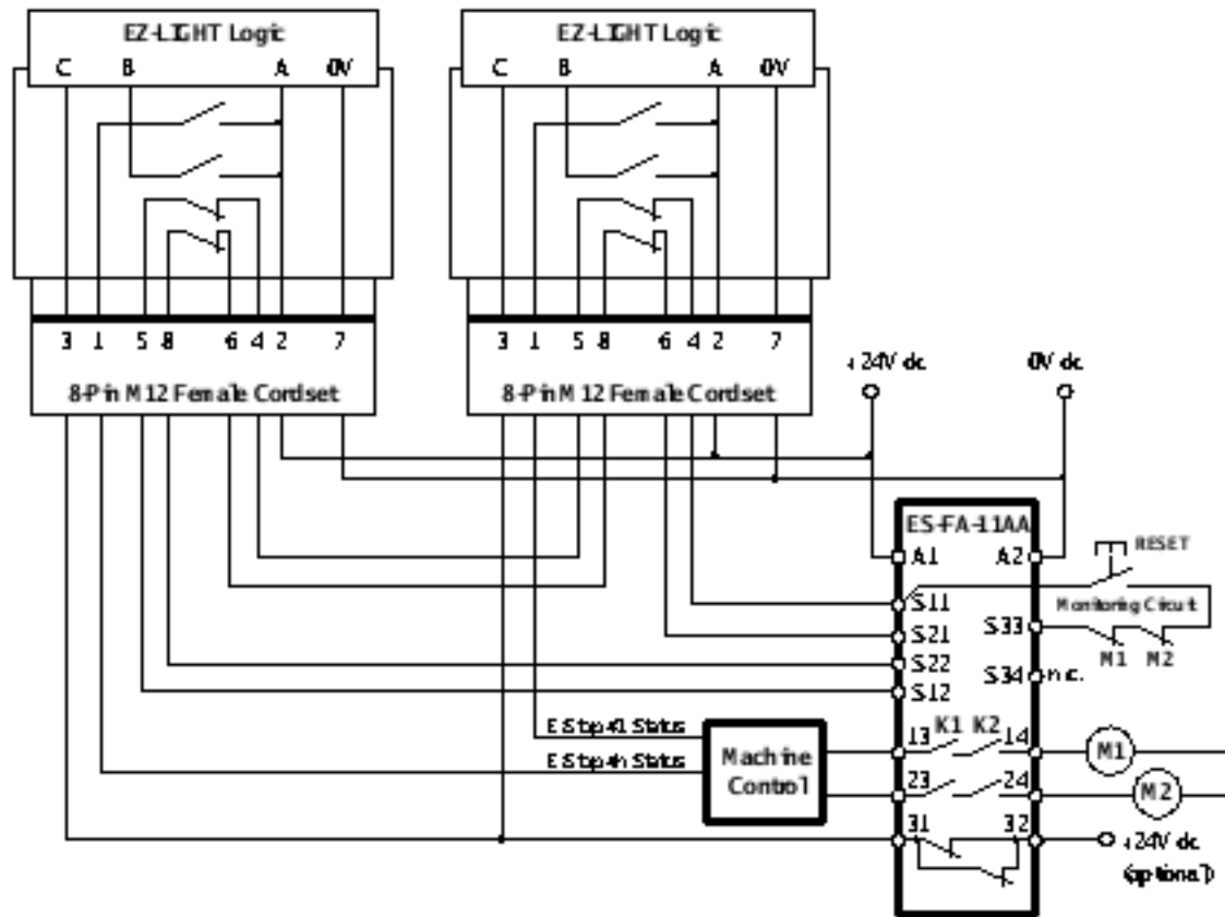
Figure 1. Illuminated models—Example wiring connection
