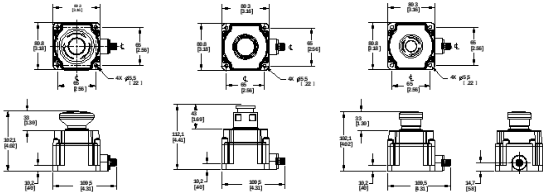
60 mm Push Button
