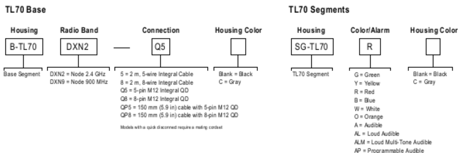
Model key for TL70 segments
