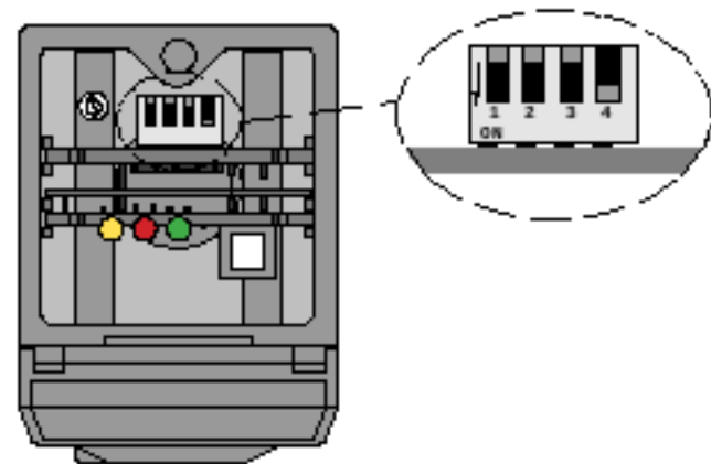
Figure 2. Q45U Programming Switches
