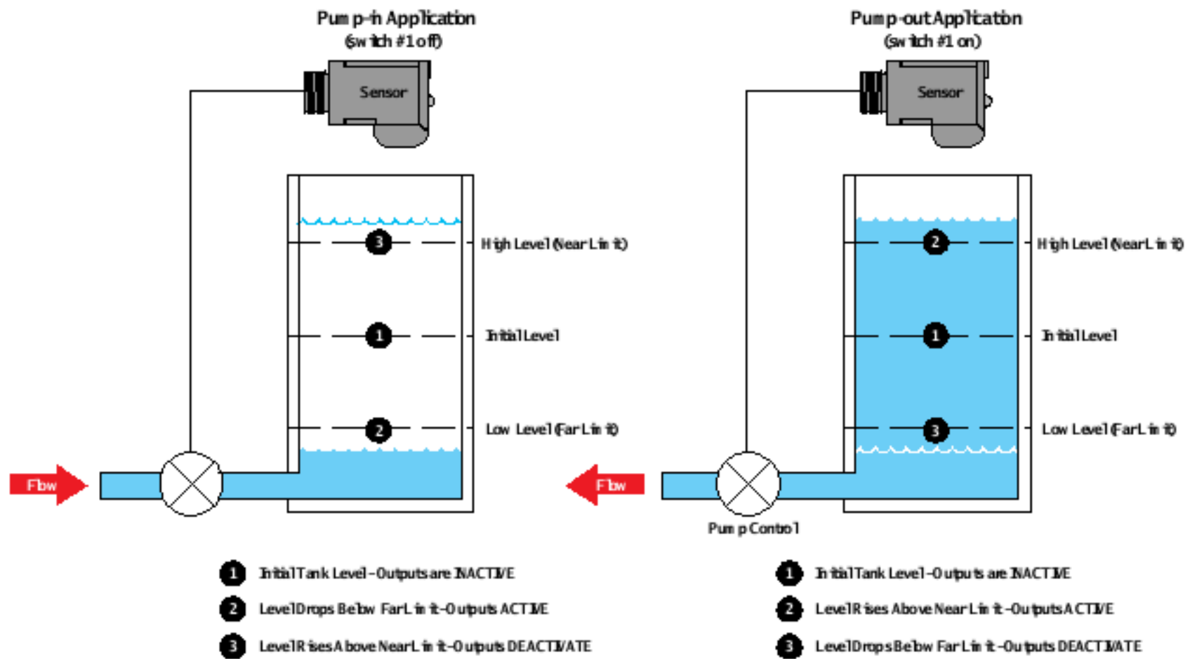
Figure 3. High/Low Control (DIP Switch 2 in On)
