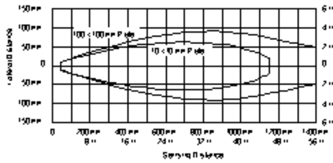
Effective Beam with Plate Target (Typical)
