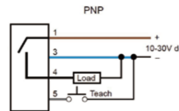
R58B接腳圖
