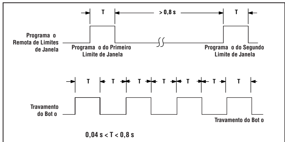
Figure 6. Timing for remote TEACH programming J Figura 6. Tempo para programação remota TEACH
