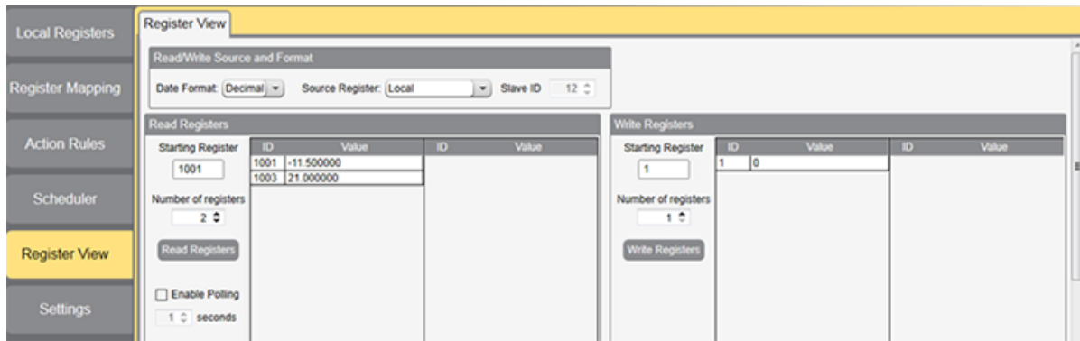
Figure 2. DXM Configurator showing the local floating point registers of the Decagon MPS-2
