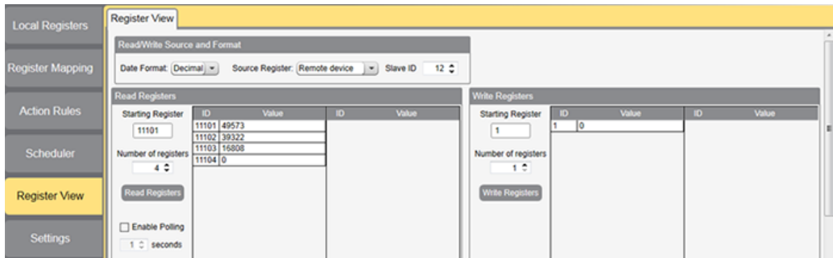
Figure 1. DXM Configurator Tool displaying the Decagon MPS-2 results registers
