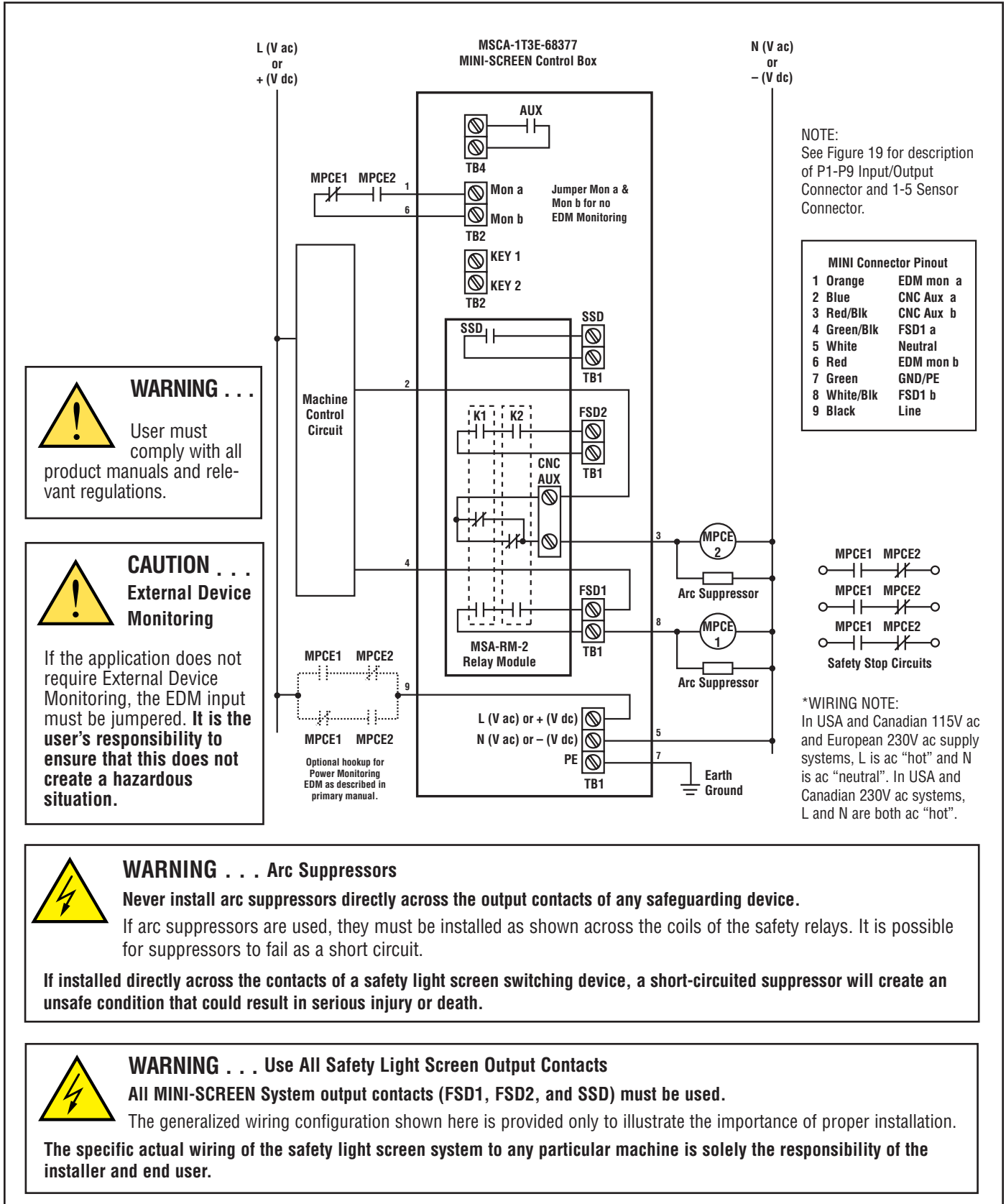
Figure 23 Replacement Figure 23(s). Generic Machine Interface, MINI-SCREEN MSCA-1T3E-68377 System with the MSA-RM-2 relay pack.
