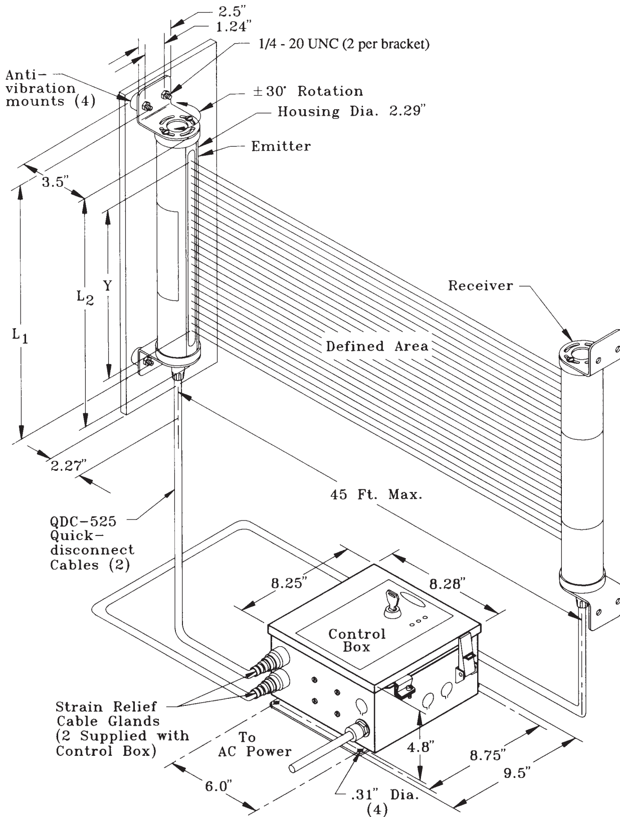
Figure 13. Dimensions, MACHINE-GUARD System
