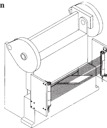
Figure 3B. Floating Blanking in Press Brake Application
