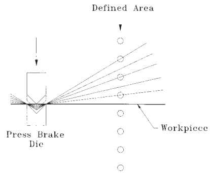
Figure 3B. Floating Blanking in Press Brake Application
