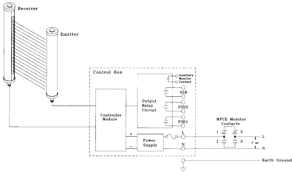
Figure 2. Banner MACHINE-GUARD System Functional Schematic
