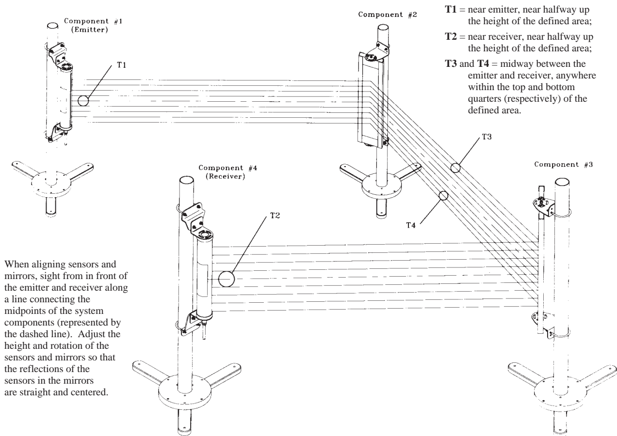
Figure 16. MACHINE-GUARD System, Alignment and Trip Test
