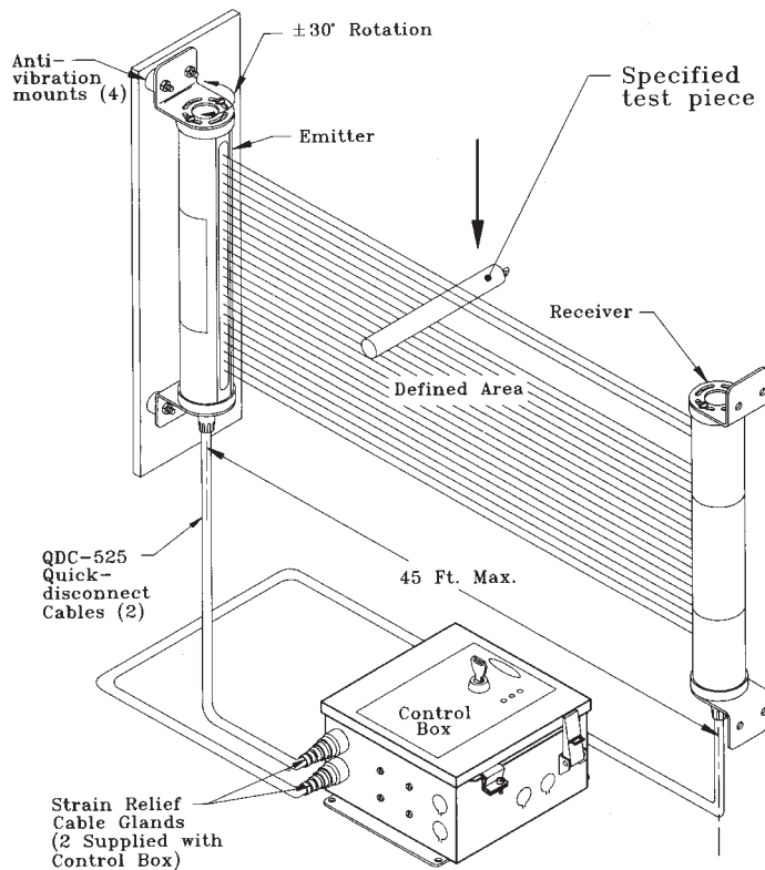
Figure 1. Banner MACHINE-GUARD System: emitter, receiver, control box, and QD-style interconnecting cable (cable is purchased separately)
