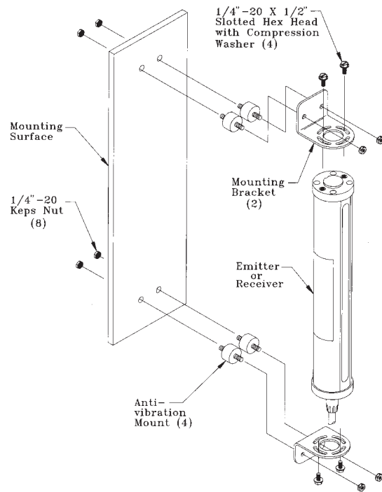
Figure 7. Emitter and Receiver Mounting (see also Figure 13, pages 18-19)
