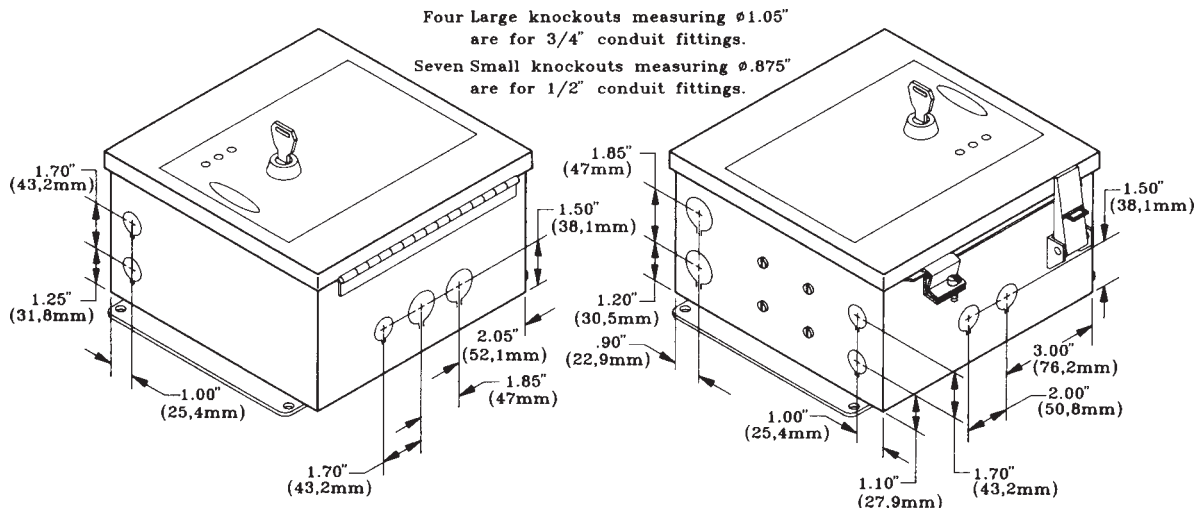
Figure 9. MACHINE-GUARD Control Box Knockout Locations
