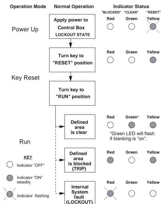
Figure 17. Operating Status LED Conditions
