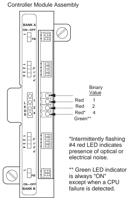
Figure 15. Interpretation of Diagnostic Indicator LEDs
