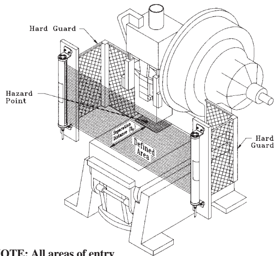
Figure 6. Hard Guarding Requirements
