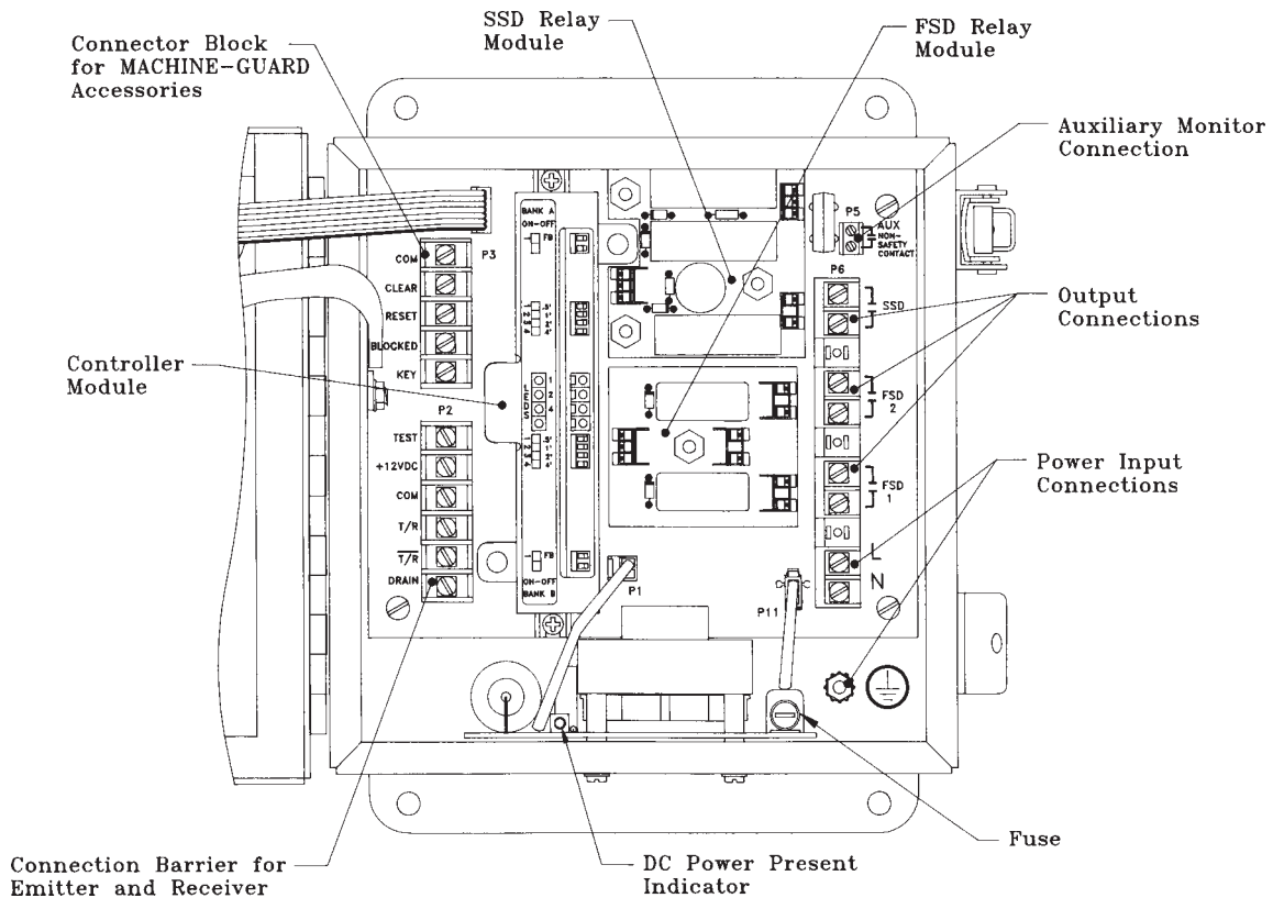
Figure 10. MACHINE-GUARD System Electrical Connections
