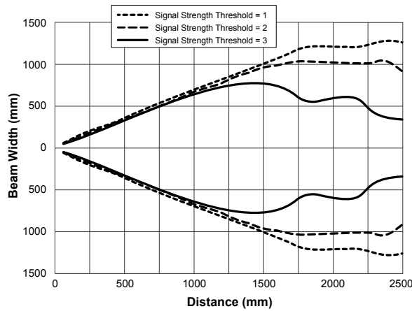
Figure 8. Typical beam pattern, in millimeters, with 250 x 250 mm Flat Metal Sheet (Radar cross section = 2000m 2 ) and various signal strength thresholds
