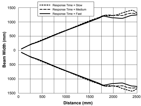
Figure 9. Typical beam pattern, in millimeters, with 250 x 250 mm Flat Metal Sheet (Radar cross section = 2000m 2 ) and various response times
