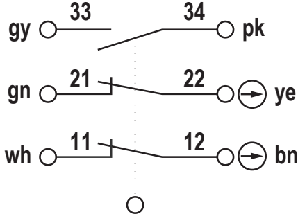
Contact Configuration (Gate Closed State) for Cabled Models
