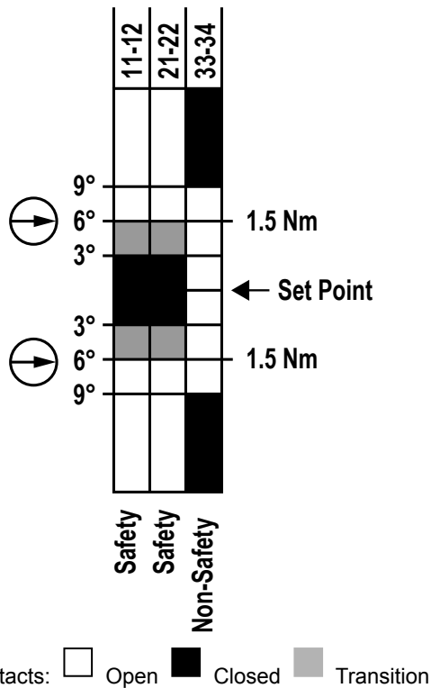
Switching Diagram
