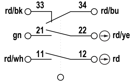
Contact Configuration (Gate Open State) for Quick Disconnect Models
