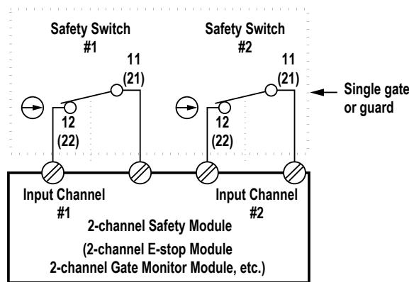
Connect two redundant safety switches per interlock guard to an appropriate 2-channel input safety module
