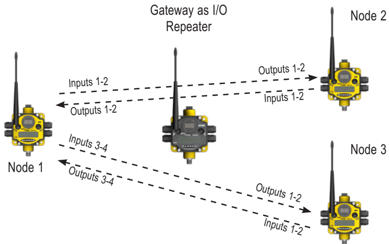
Configured input/output mapping
