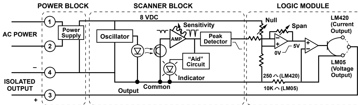
Figure 5. Functional schematic
