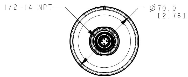
VIEW Z-Z
