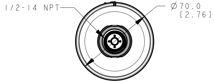
VIEW Z-Z
