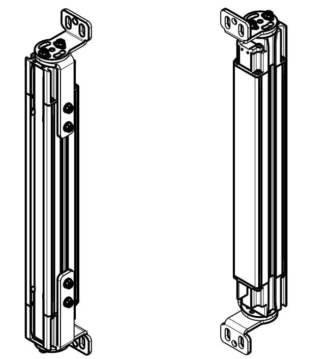
ISOMETRIC VIEW SCALE 1:4
