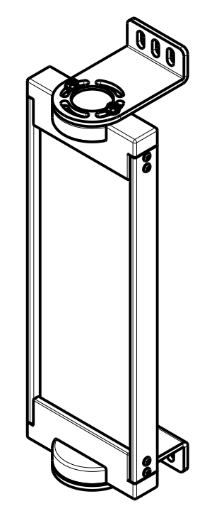
ISOMETRIC VIEW SCALE 1:4
